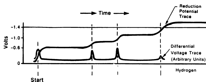
FIG. 1 Ideal Reduction Behavior of Oxide and Sulfide Films on Copper (from Ref 1)
