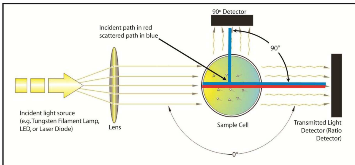
FIG. 2 Single Beam Design Ratio Nephelometer (Single Beam Design)
