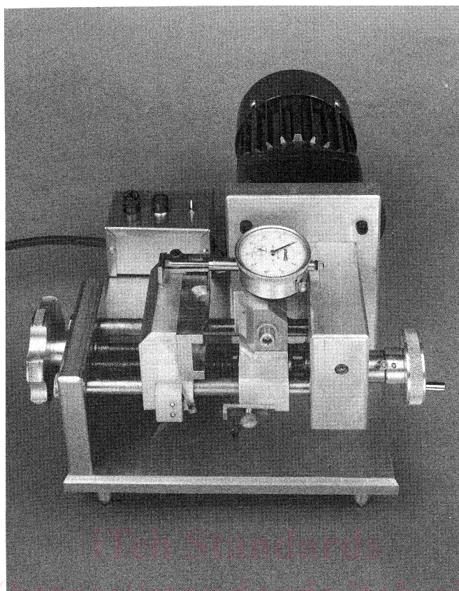
FIG. 2 Notching Machine
