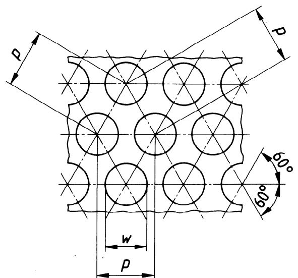
Figure 1 — Arrangement of round apertures
