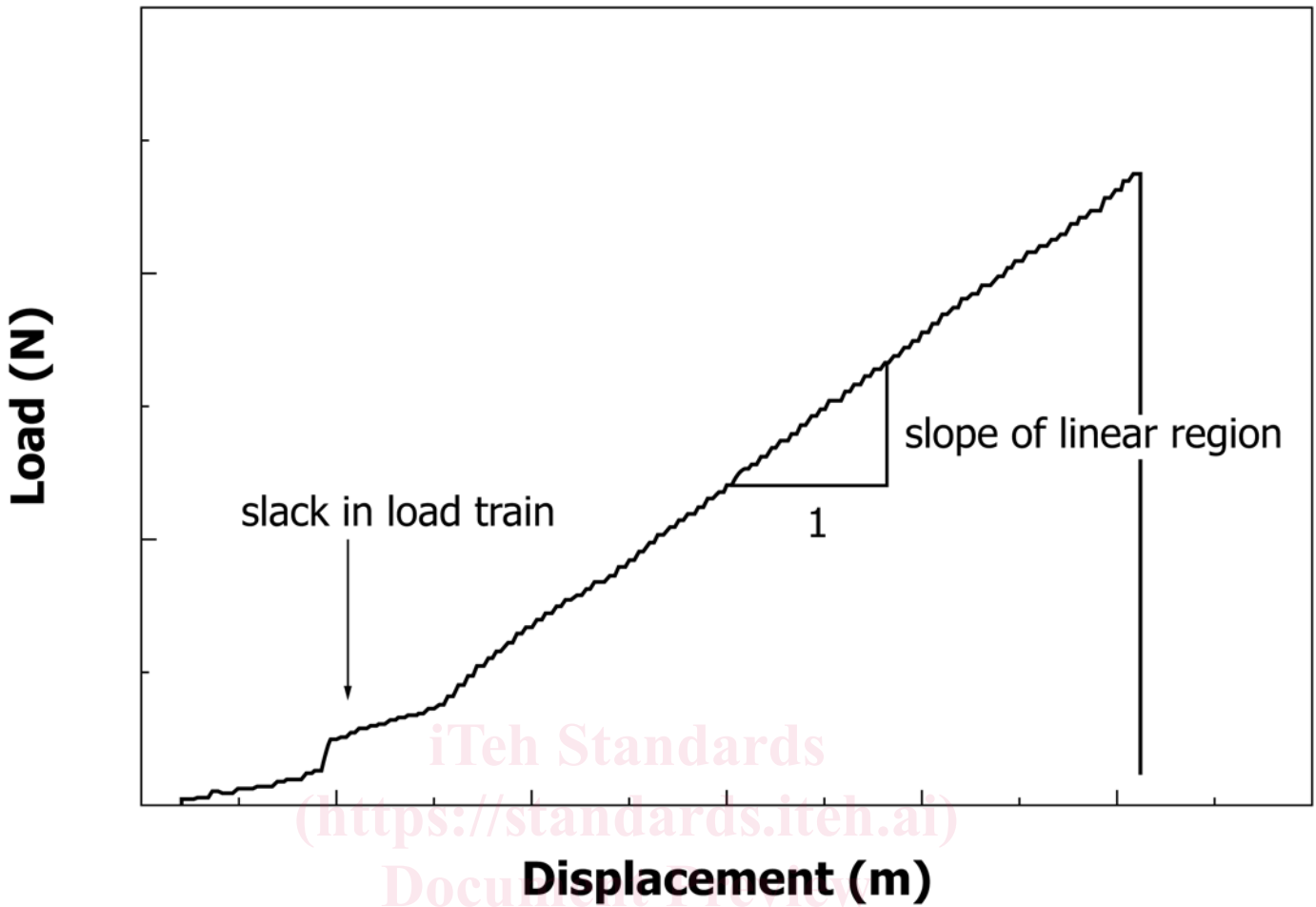
FIG. 5 Typical Load versus Cross-head Displacement Curve
