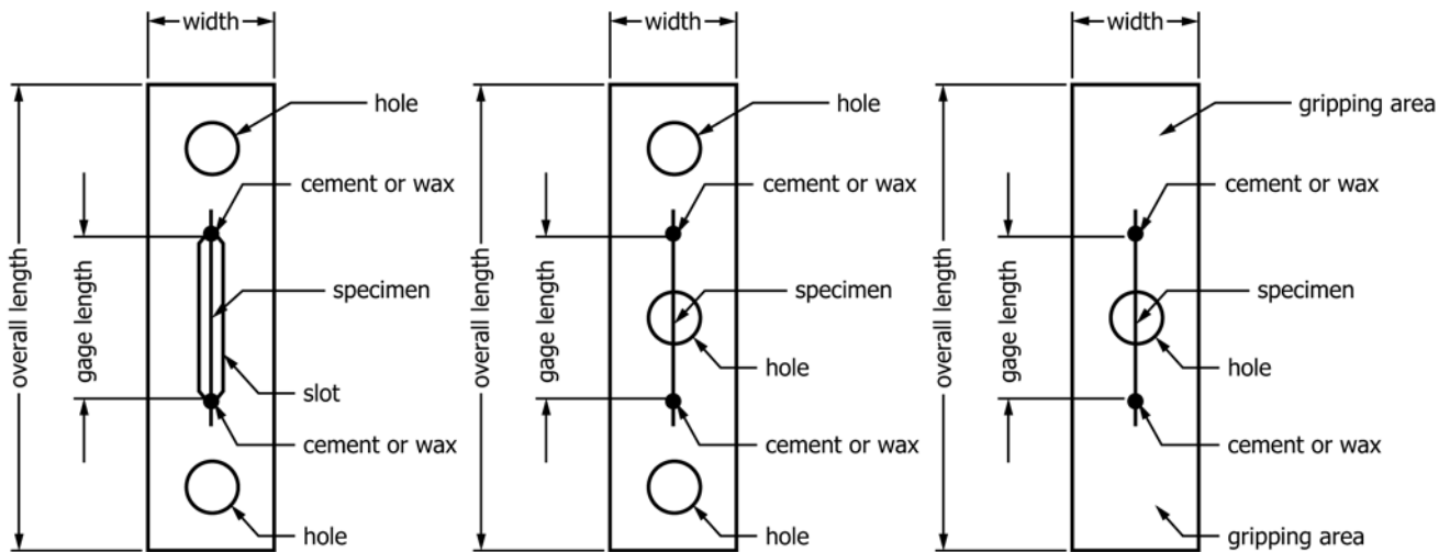
FIG. 3 Mounting Tab
