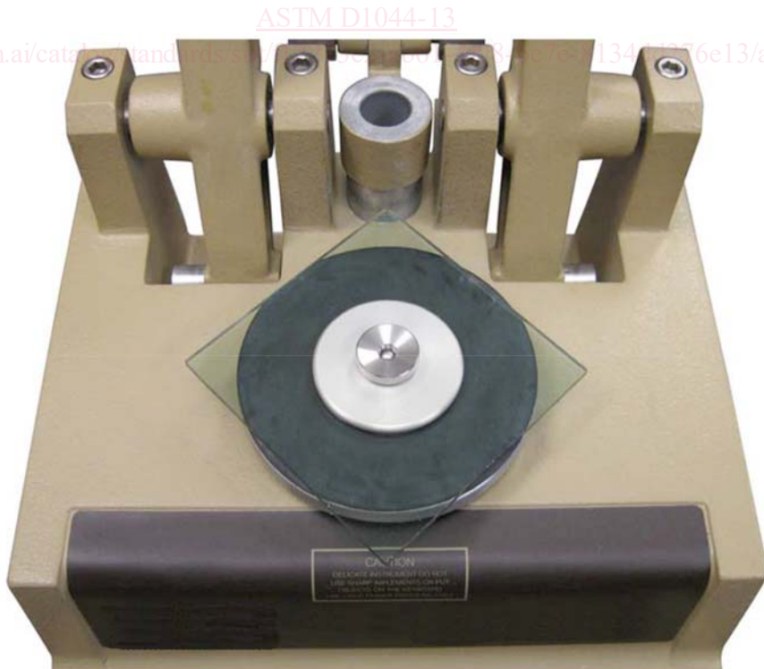
FIG. 3 Specimen Mounting
