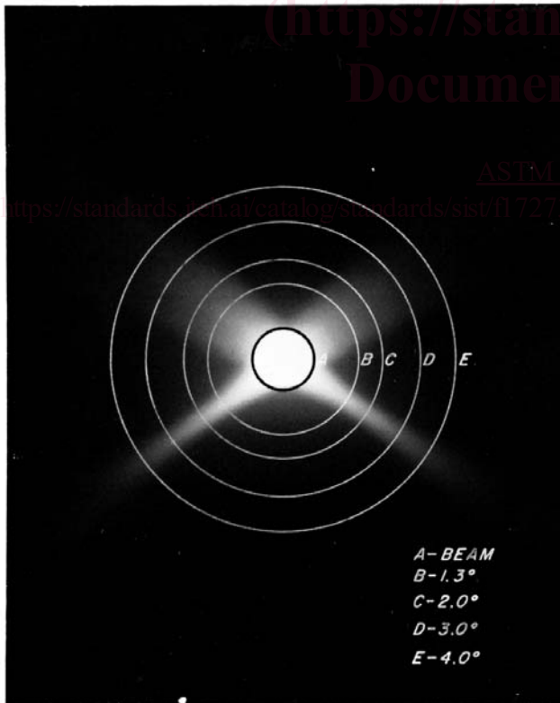
NOTE 1—This photograph shows light pattern of the scattering from the surface of a Taber abraded specimen. The circles show how increasing the 1.3° dark annulus dramatically changes the amount of light impacting the sphere wall.
