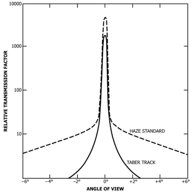
NOTE 1—This graph shows goniophotometric curves for Taber abraded tracks. The specular angle of transmission is at 180°.
