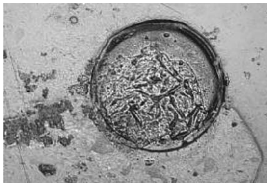
FIG. X1.1 Digital Photograph of Acid Etch Produced During Field Exposure (Jacksonville, FL, 50 × magnification)
