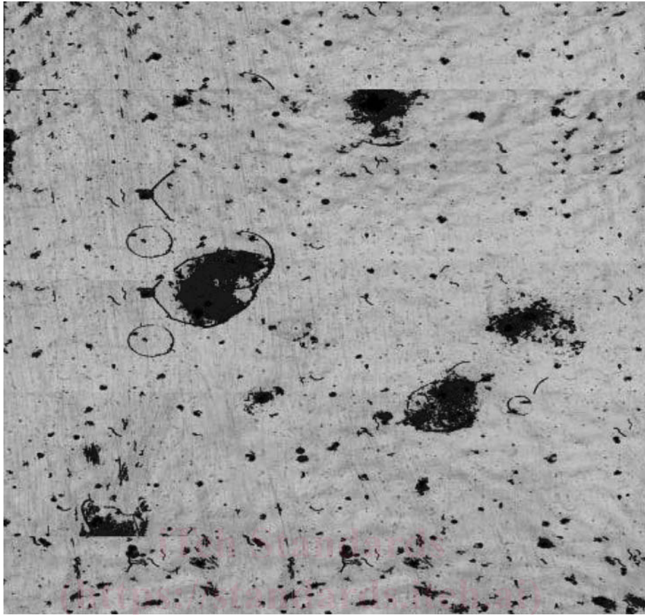
FIG. X1.3 Digitally Enhanced Photograph of Acid Etch Produced by the Exposure Described in This Standard (actual size 4 × 6 in.). 10 Rating 4.97 % Defects
