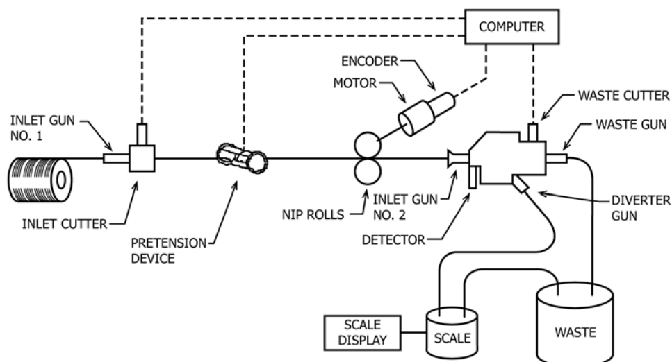
FIG. 1 Yarn String-up Diagram for ACW (Automatic-Cut-and-Weigh) Tester
