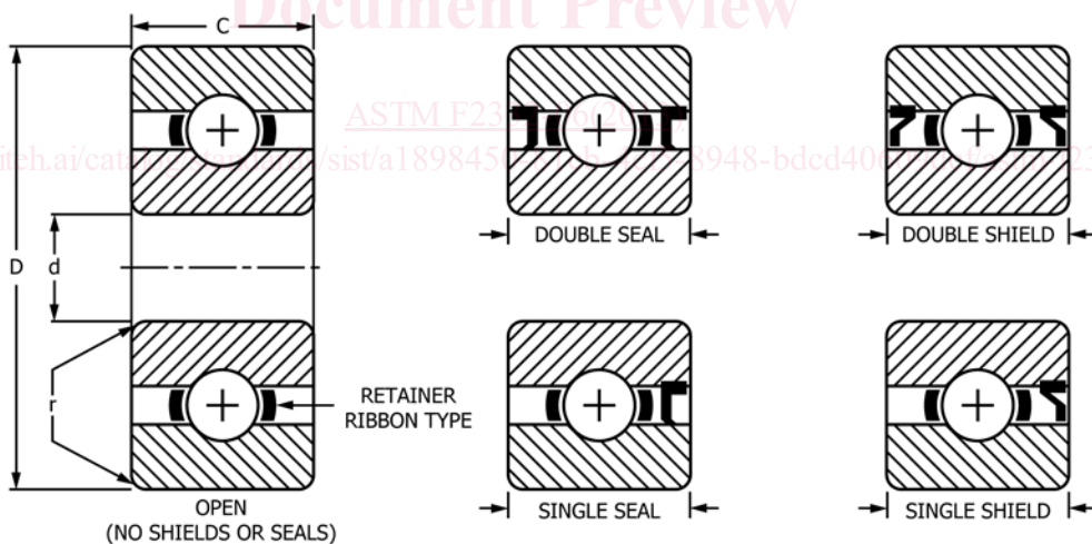
FIG. A2.1 Bearing Configuration
