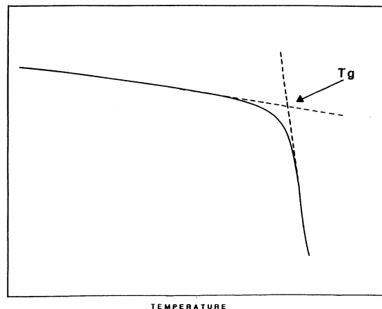
FIG. 1 Storage Modulus
