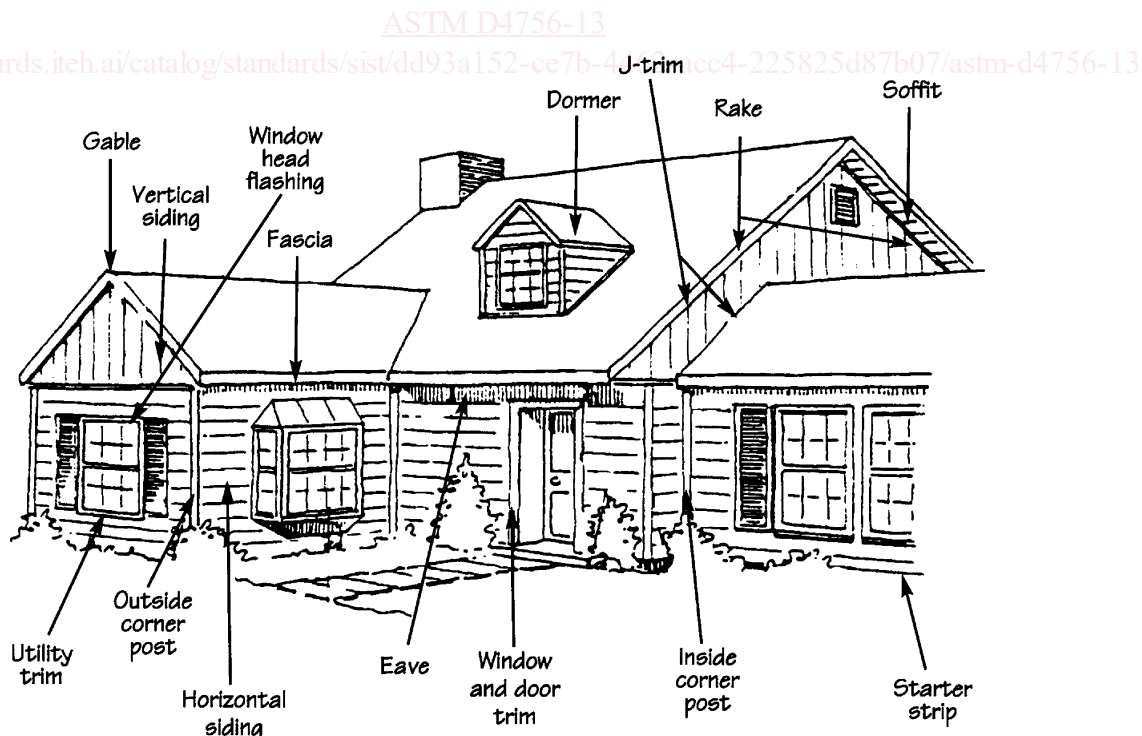
FIG. 1 Terminology for Buildings, Siding and Accessories
