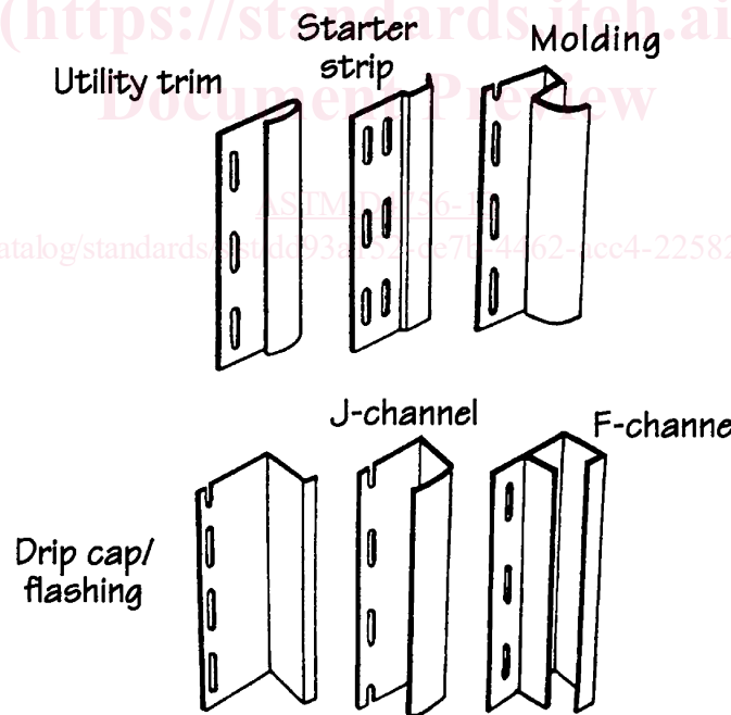
FIG. 5 Typical Siding Accessories
