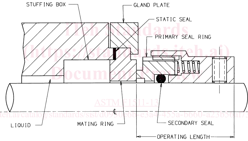
FIG. 3 Single Seal—Outside Mounted Classification Type B Grade 1
