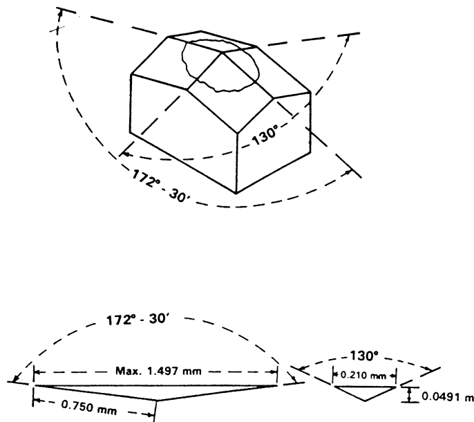
FIG. 12 Knoop Indenter Showing Maximum Usable Dimensions
