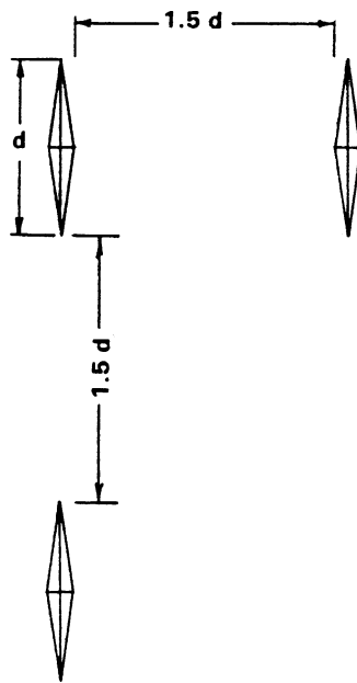
FIG. 23 Closest Permitted Spacing for Knoop Indentations
