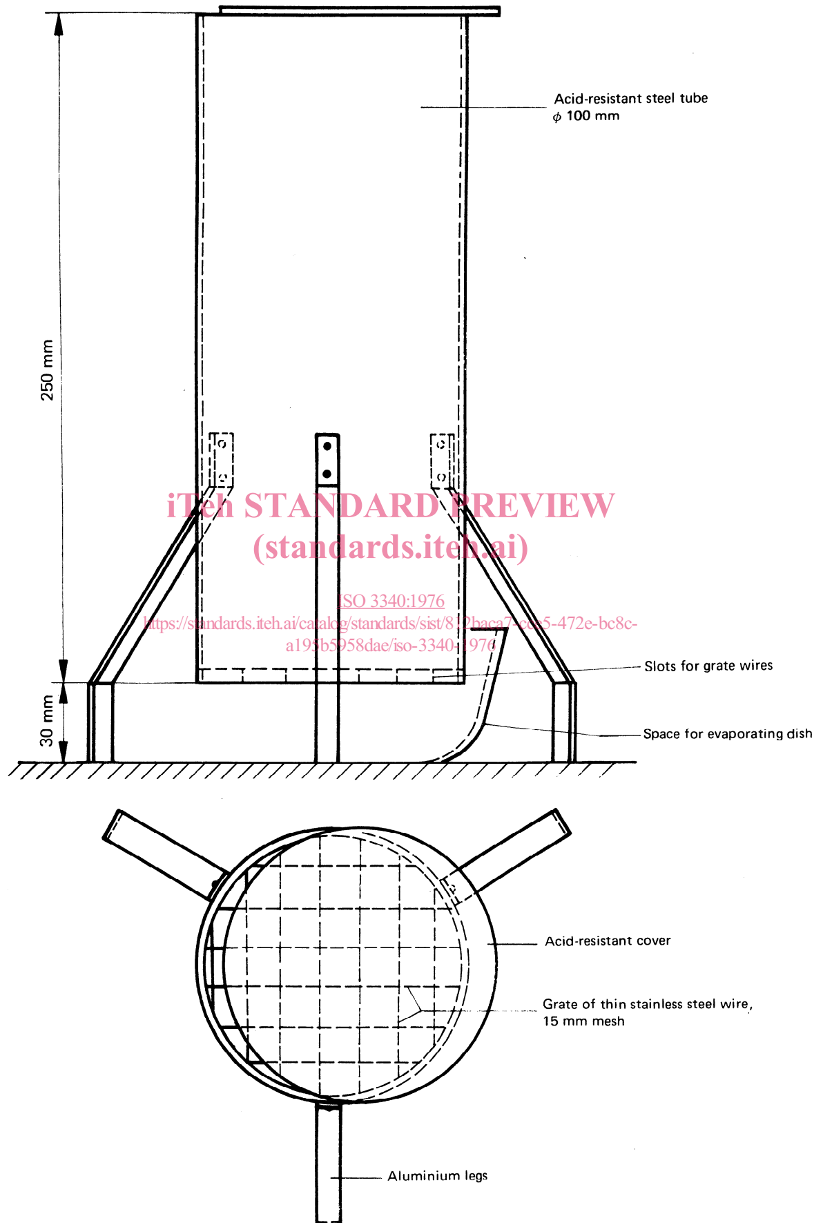
FIGURE – Tubular hearth (7.2)
