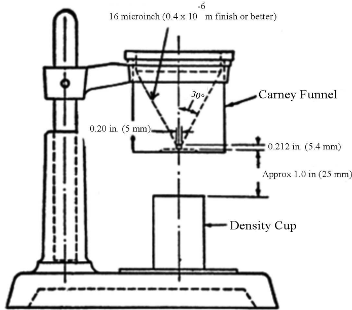
FIG. 1 Carney Flowmeter Funnel and Stand
