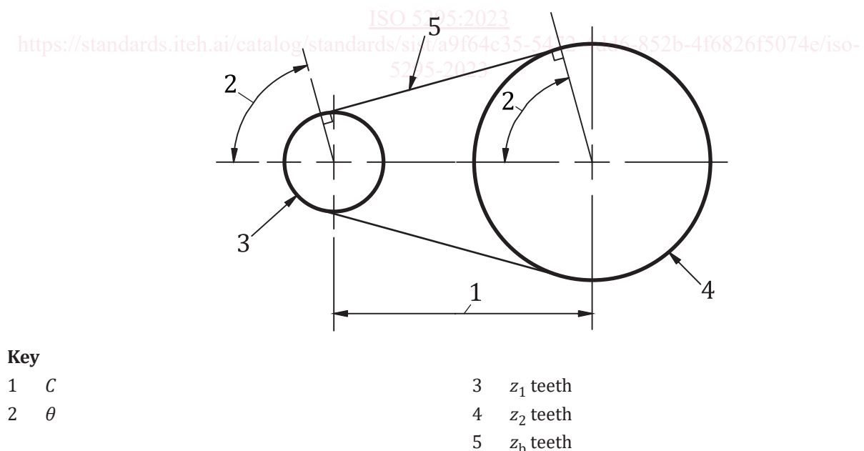
Figure 1 — Centre distance
