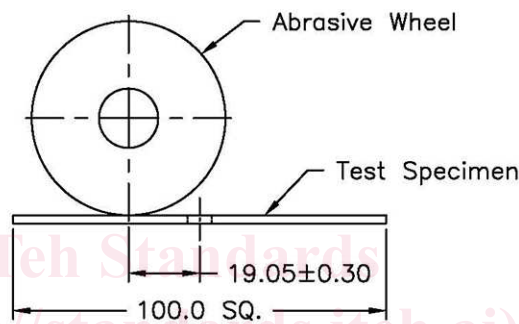
dimensions in millimeters FIG. 2 Central Axis of the Turntable
