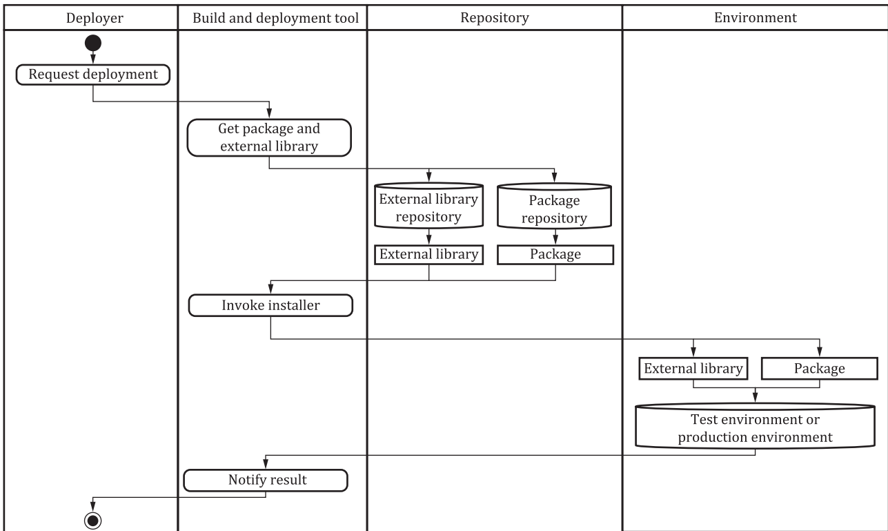
Figure 5 — Activity diagram of deployment
