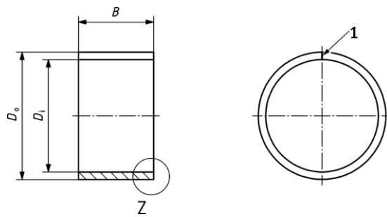
a) Type C cylindrical bush
