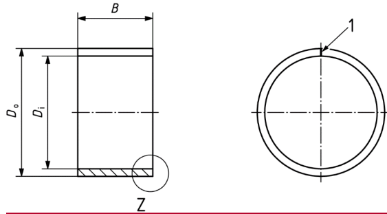
a) Type C cylindrical bush
