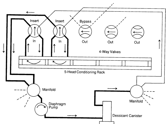
FIG. 2 Conditioning System
