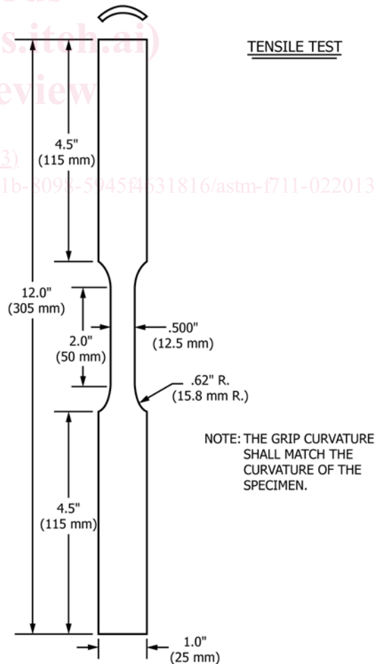
FIG. 1 Tension Test
