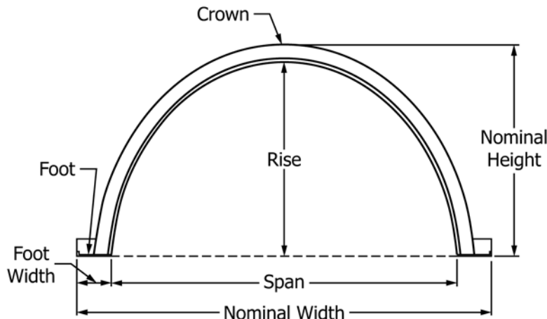
The model chamber shown in this standard is intended only as a general illustration. Any arch-shape chamber configuration is permitted, as long as it meets all the specified requirements of this standard.
