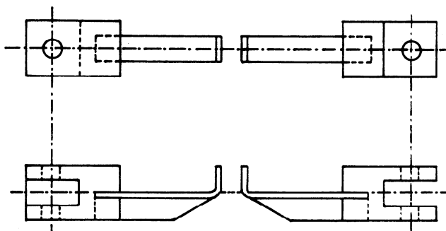
FIGURE 2 — Test piece holders
