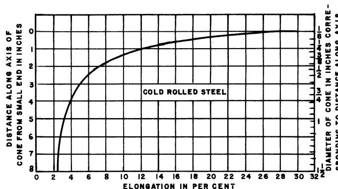
FIG. 2 Distance Along Cone and Corresponding Mandrel Size versus Percent Elongation for Specimens on Cold-Rolled Steel 0.8 mm [ 1/32 \text{ in.} ] in Thickness
