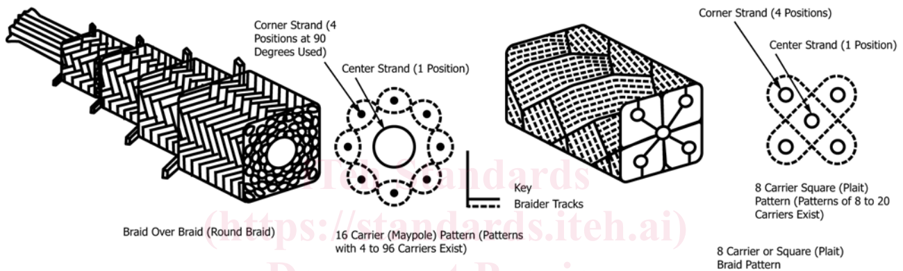
Interlocking and Square Plait Versus Braid-Over-Braid Patterns
