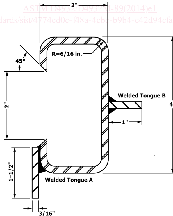
FIG. 1 Nailers Holding Jig, 100 mm (4 in.) [4 in.] Long, Cold-Formed Carbon Steel
