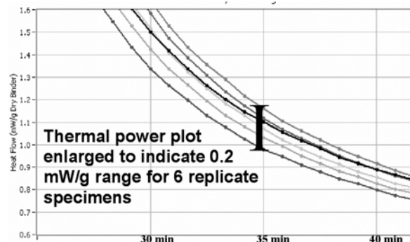
FIG. 3 Illustration of Estimated Time to Reach Thermal Equilibrium Using Six Replicate Specimens
