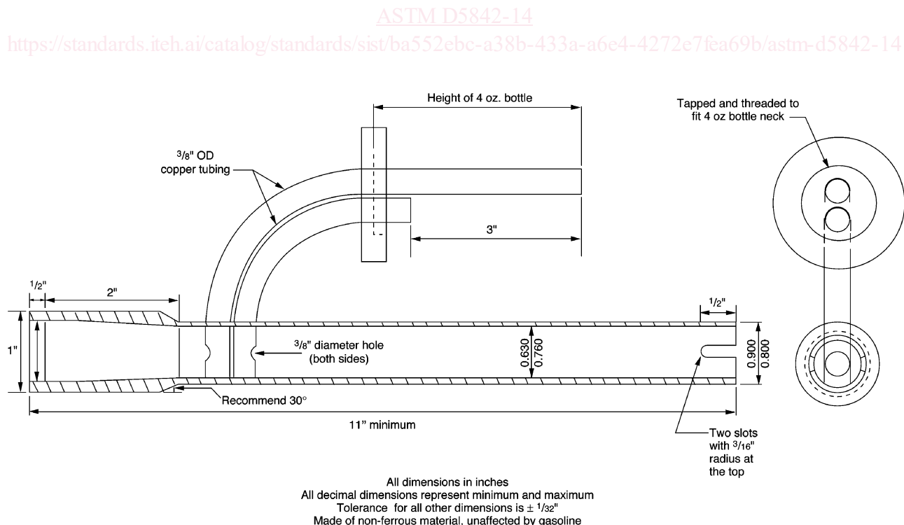
FIG. 1 Nozzle Extension for Nozzle Sampling with 4 oz Bottle
