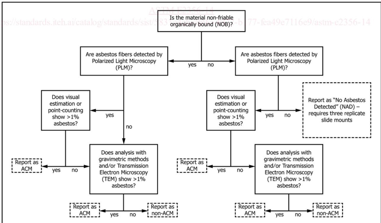
FIG. 2 Protocol for Analysis of Bulk Samples
