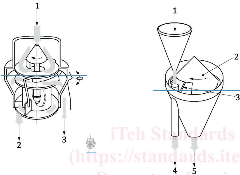
a)Figure 2 — Examples of dividers — Rotating disc type b) Rotating cone type
