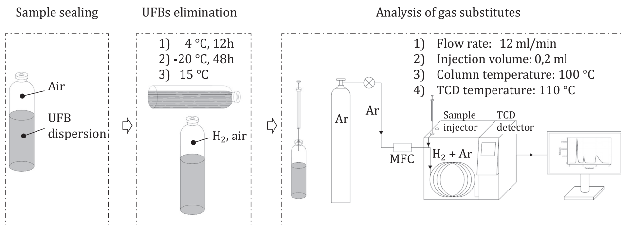
Figure 2 — General view of gas chromatography system
