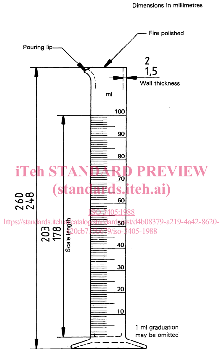
Figure 4 – Graduated cylinder (100 ml in 1 ml graduations, tolerance \pm 1,0 ml)
