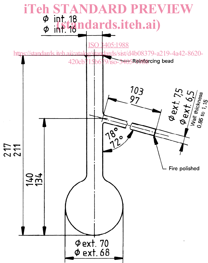
Figure 1 — Distillation flask
