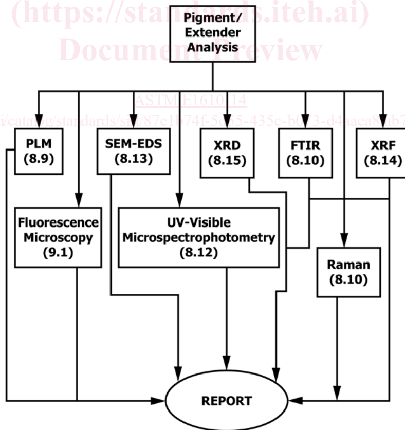
FIG. 3 Scheme for Forensic Paint Examinations
