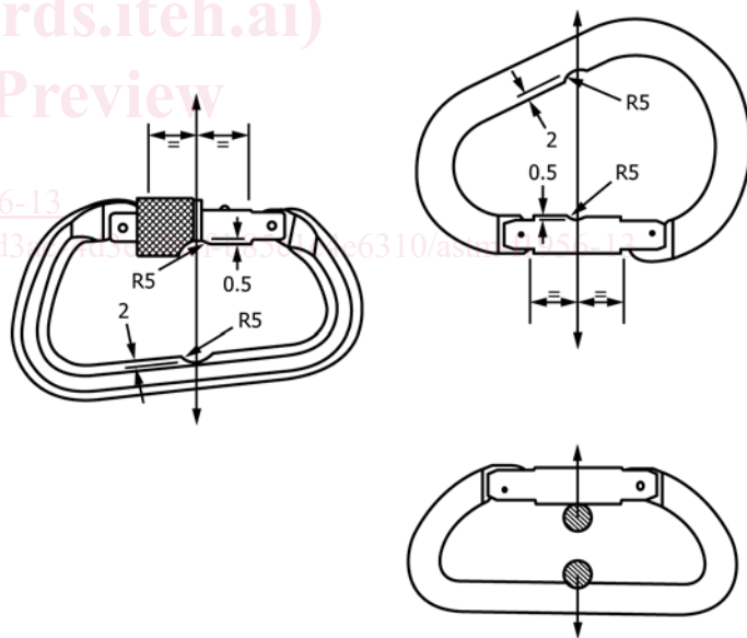
FIG. 2 Test Fixture
