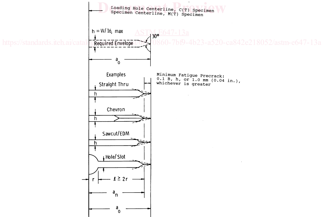
FIG. 1 Notch Details and Minimum Fatigue Precracking Requirements
