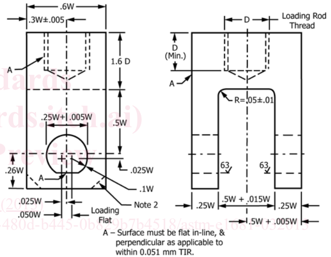
NOTE 1—Pin diameter = 0.24 W (+0.000W/-0.005W) . For Specimens a with \sigma_{vs} > 1379 \text{ MPa} the holes in the specimen and in the clevis may be 0.3W (+0.005W/-0.000W) and the pin diameter = 0.288W (+0.000W/-0.005W) NOTE 2—Corners of the clevis may be removed if necessary to accommodate a clip gage FIG. 2 Tension Test Clevis Design
