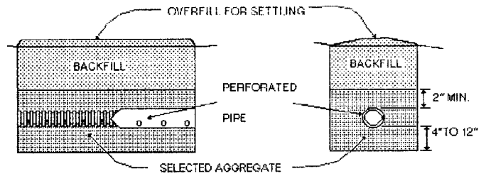
FIG. 1 Gravel Leach Trench
