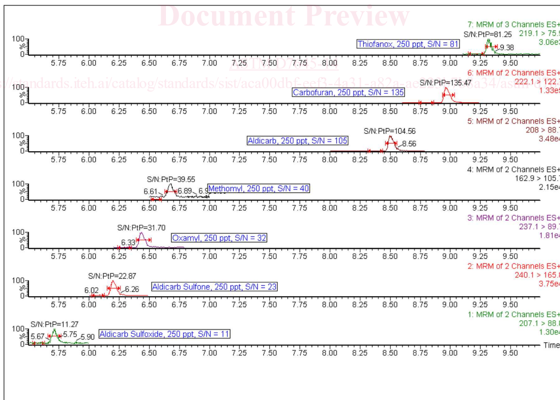
FIG. 2 Example Confirmatory SRM Chromatograms Signal/Noise Ratios
