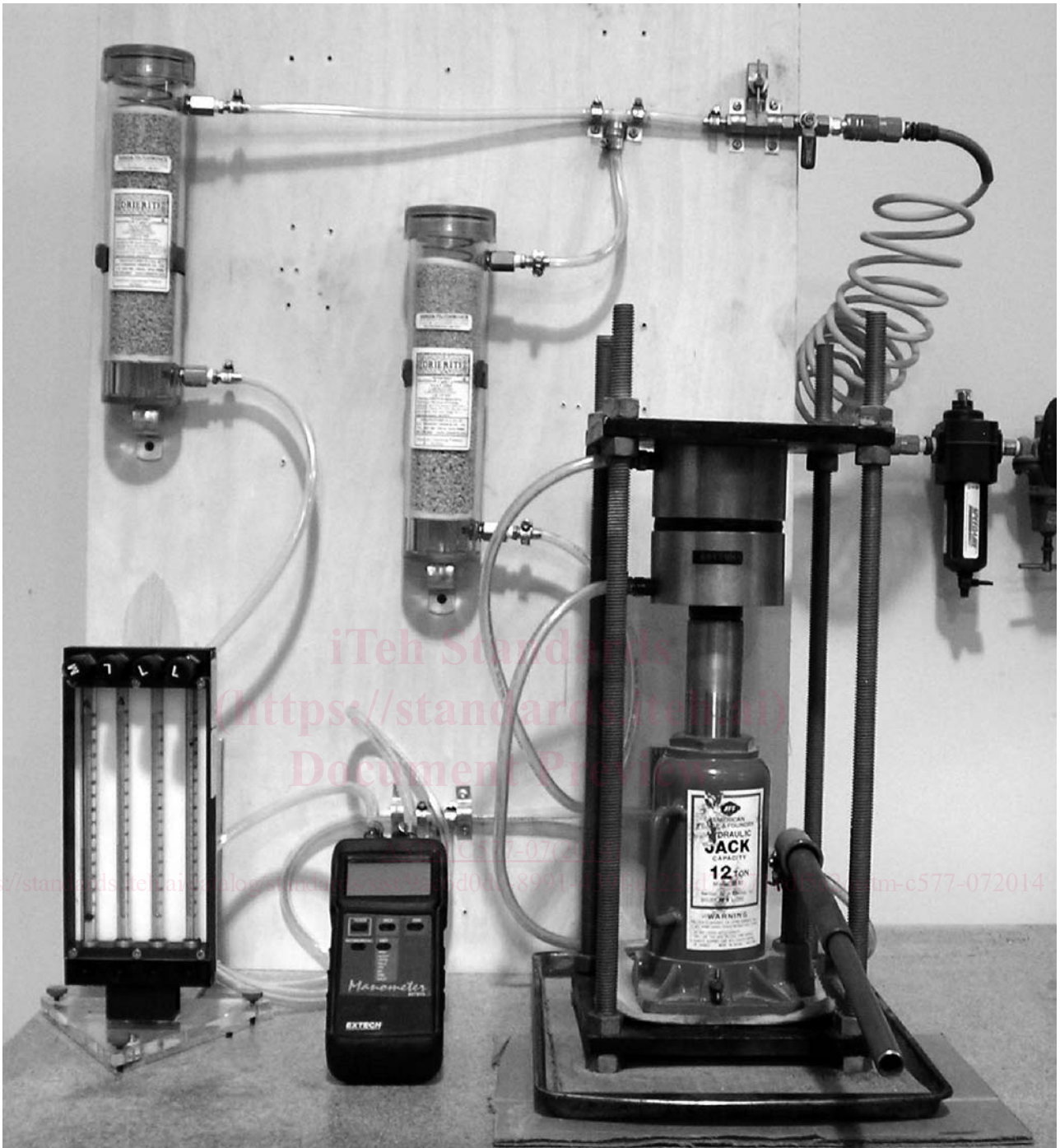
FIG. 1 Permeability Apparatus
