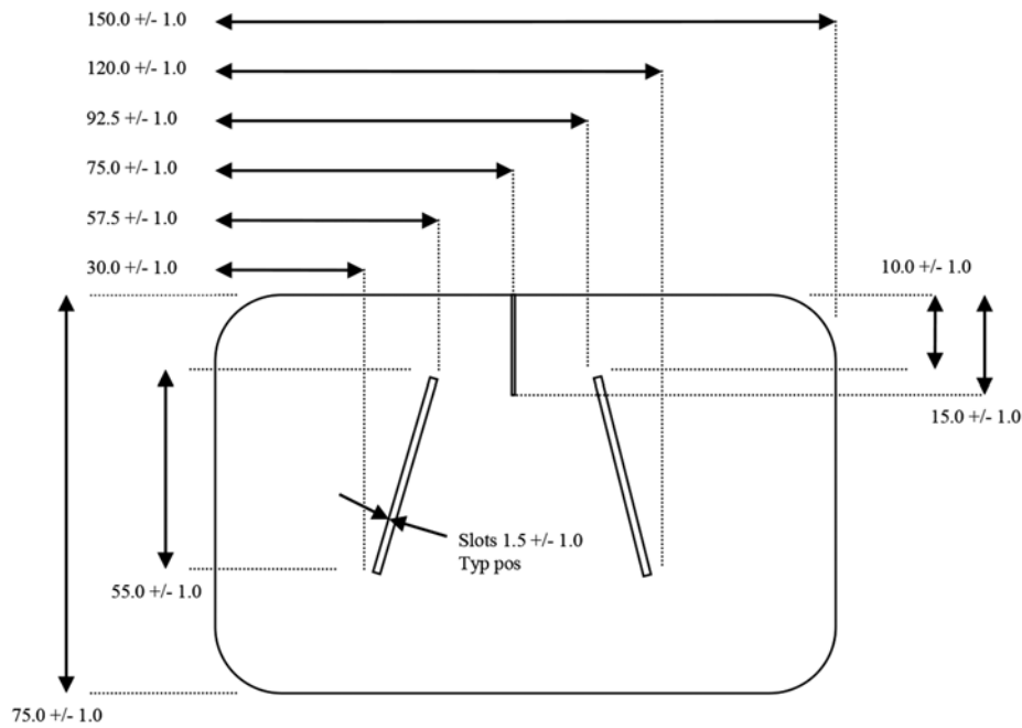
FIG. 2 Templates for Cutting and Marking Trapezoid Test Specimens
