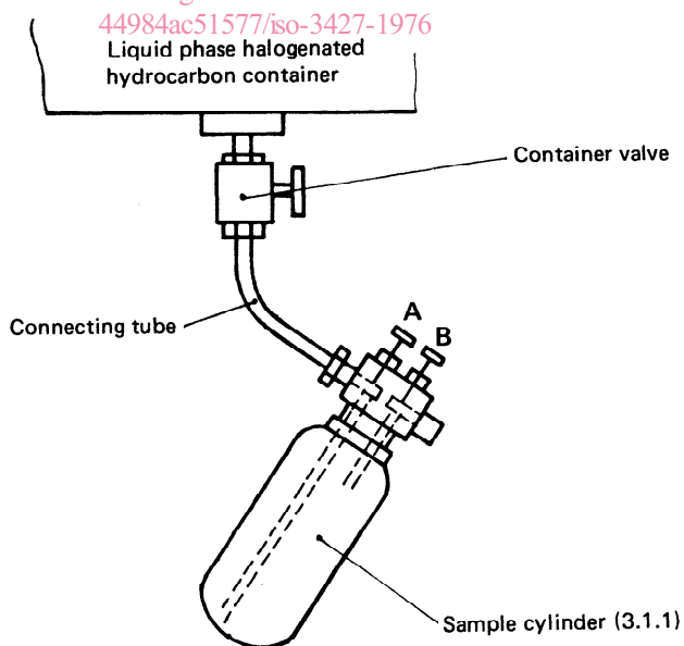
FIGURE 2 – Assembly using a type (a) sample cylinder
