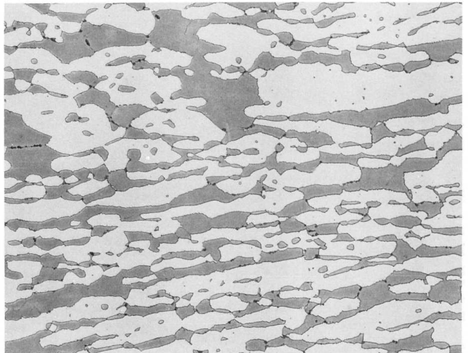
FIG. 3 Possibly Affected Structure in S31803: (a) Longitudinal Section and (b) Transverse Section (500x Magnification Before Reproduction)
