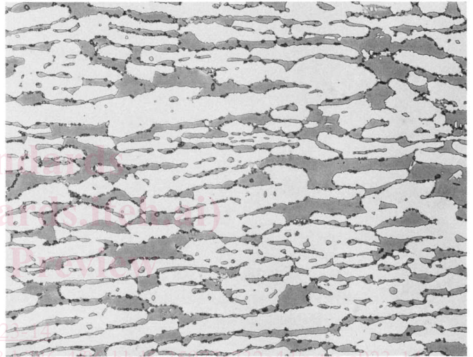
FIG. 5 Affected Structure in 8a S31803: (a) Longitudinal Section and (b) Transverse Section (500x Magnification Before Reproduction)
