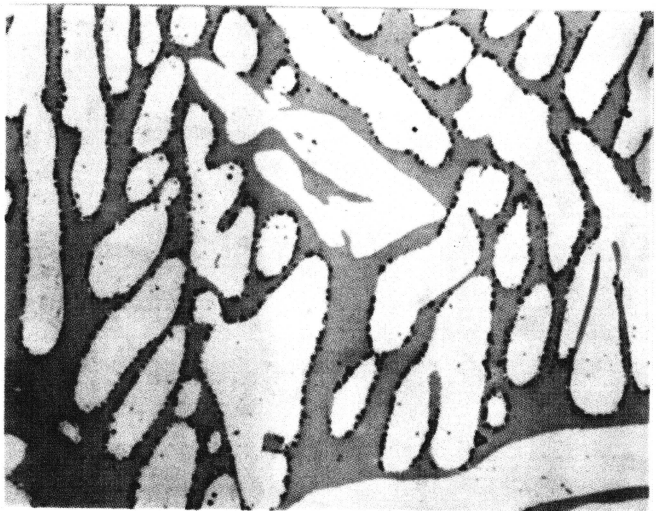
FIG. 6 J92205: Affected Structure (400x Magnification)
