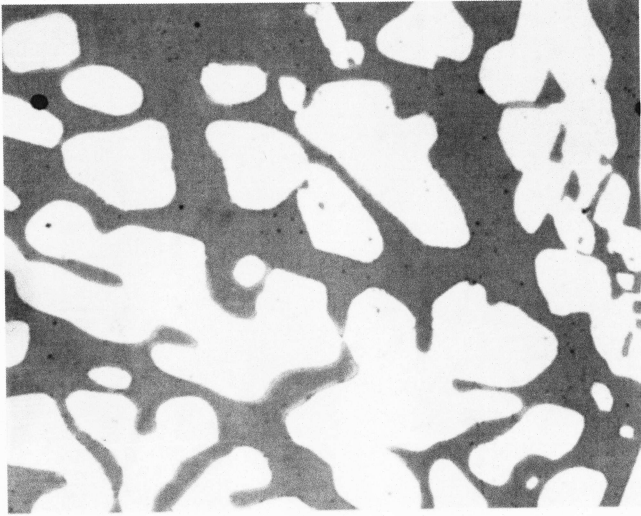
FIG. 4 (a) J92205: Possibly Affected Structure-Statically Cast (400x Magnification)
