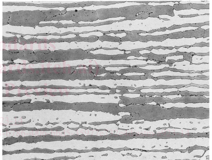
FIG. 2 (b) J92205: Unaffected Structure-Centrifugally Cast (400x Magnification) (continued)
