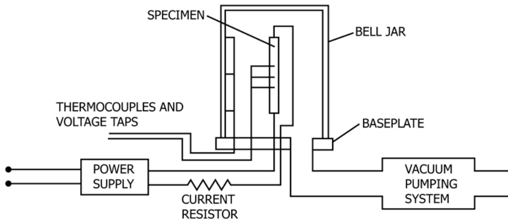
FIG. 1 System Arrangement
