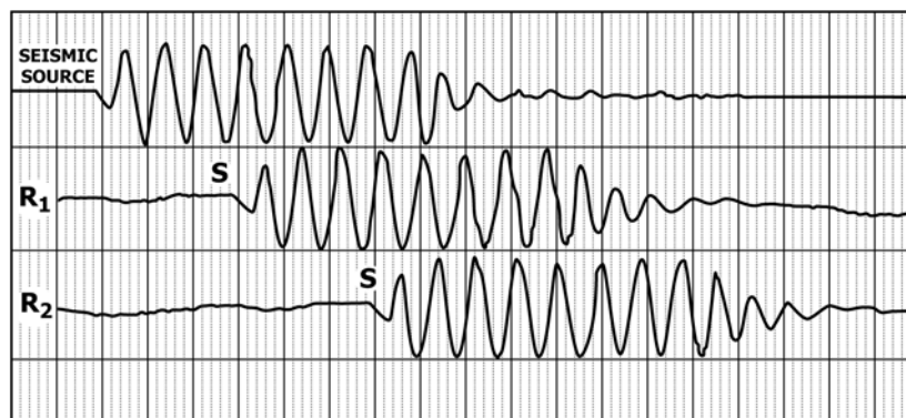
FIG. 2 Borehole Vibratory Seismic Source Time Plot (Produces S-Wave Train Only)
