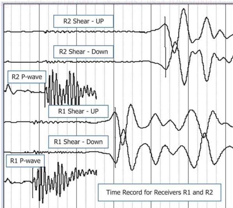
FIG. 1 Reversible Impulse Seismic Source Time Plot Showing Both P-Wave and S-Wave Trains
