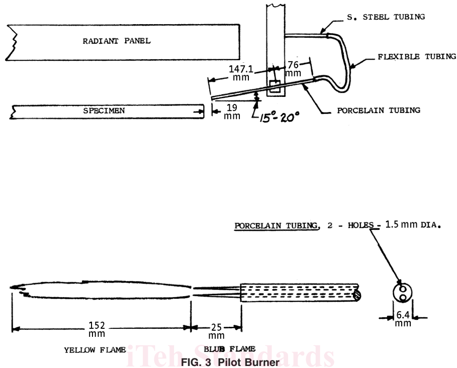
FIG. 3 Pilot Burner
