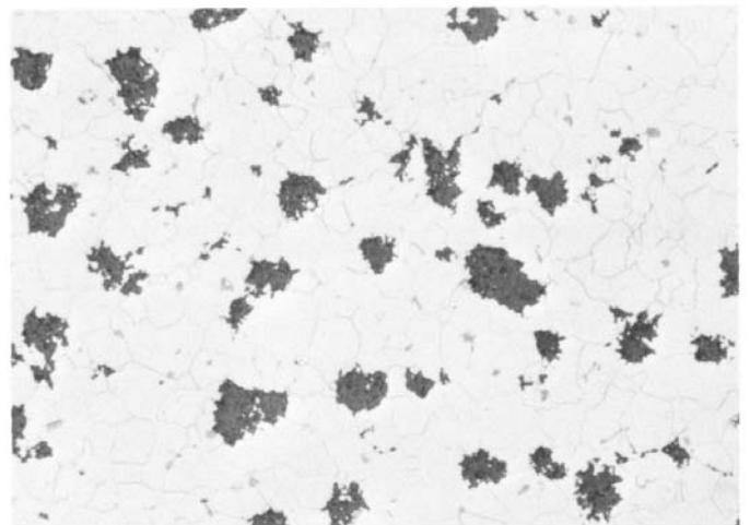
FIG. X1.1 Grade M3210, Approximately HB 143 (100x)
