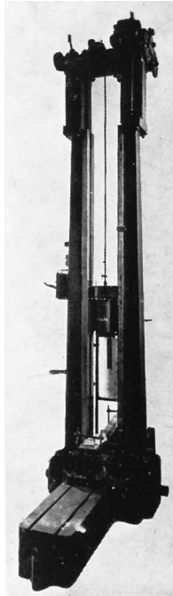
FIG. 11 Hatt-Turner Impact Machine, Illustrating Test Method of Conducting Impact Bending Test
