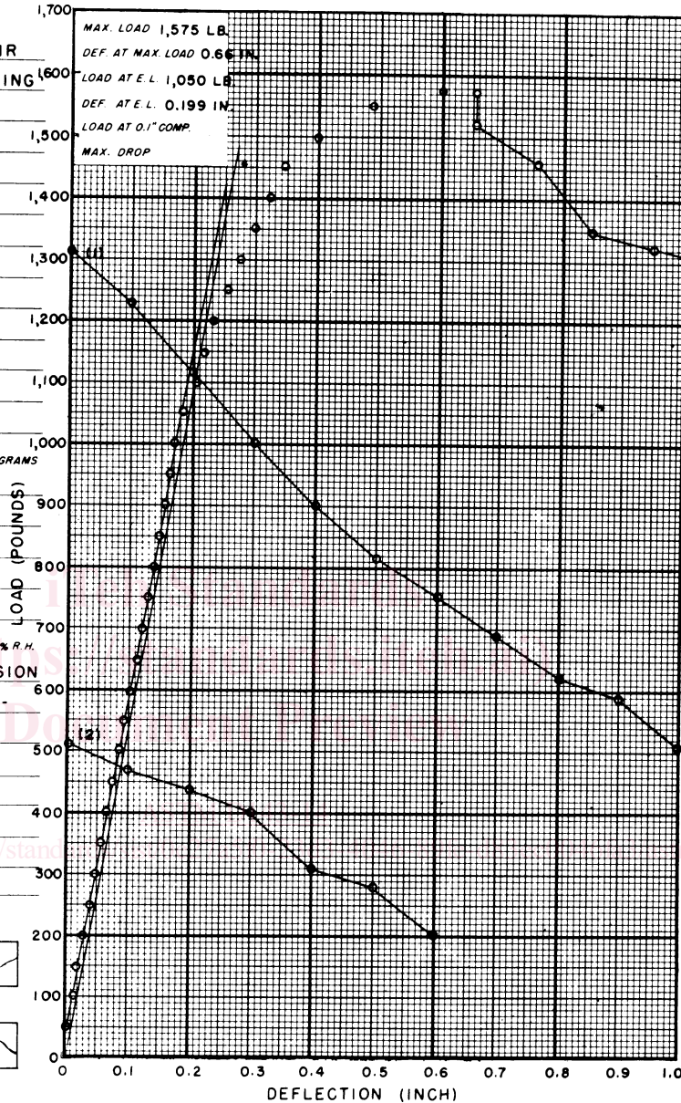
FIG. 5 Sample Data Sheet for Static Bending Test
