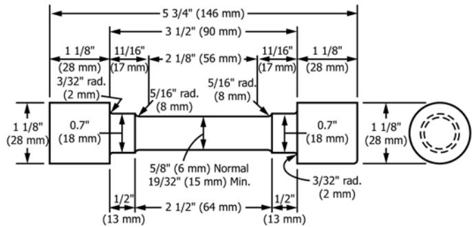
FIG. 2 Alternative Unmachined Tension Test Specimen
