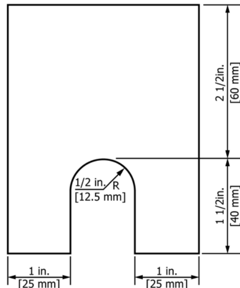
NOTE 1—The length of the keel block shall be 6 in. [152 mm] FIG. 2 Keel Block for Test Coupons
