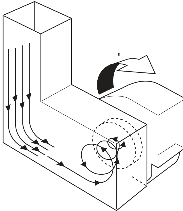
Figure 2 — Vortex at fan inlet ( https://standards.iteh.ai )
